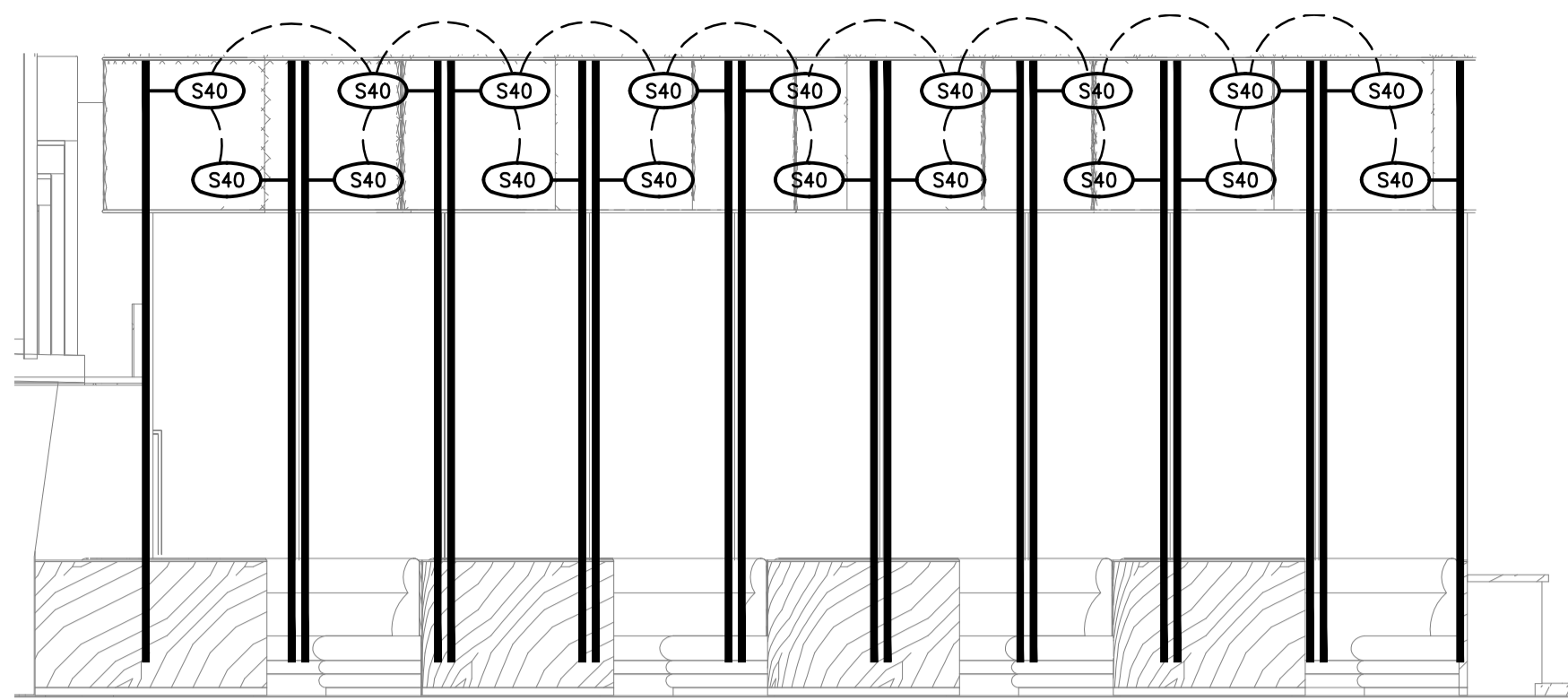
DETAIL C14 BISTRO GREENWALL SCALE 1:50
